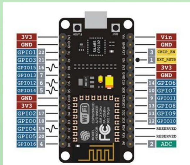
Figure 6. NodeMCU pin structure (Taştan, 2019).
